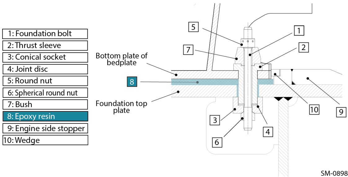
Figure 5: Epoxy resin as an interface between the engine bedplate and foundation top plate
