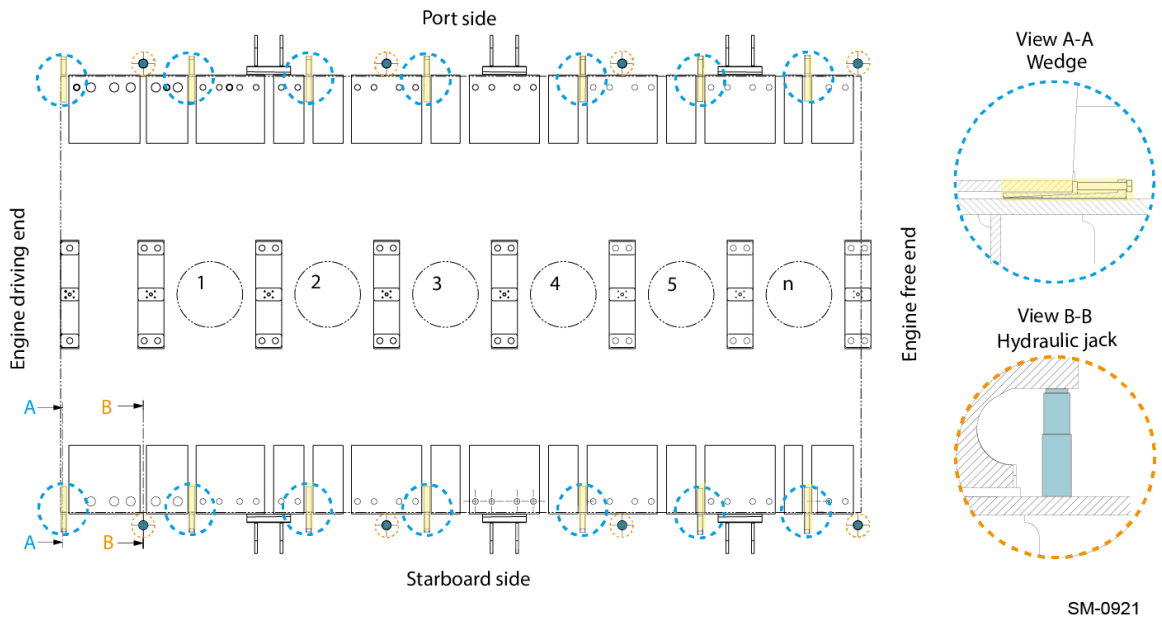
Figure 15: Engine alignment by wedges and/or shims with hydraulic jacks
