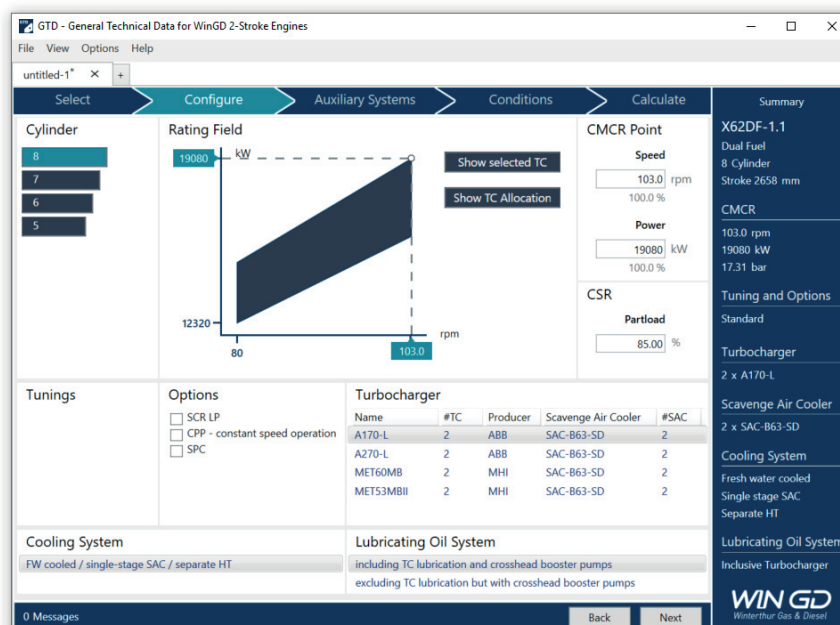
Figure 0-1 GTD screenshot
