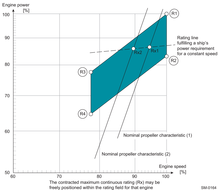
Figure 2-1 Rating field for the X62DF-1.1
