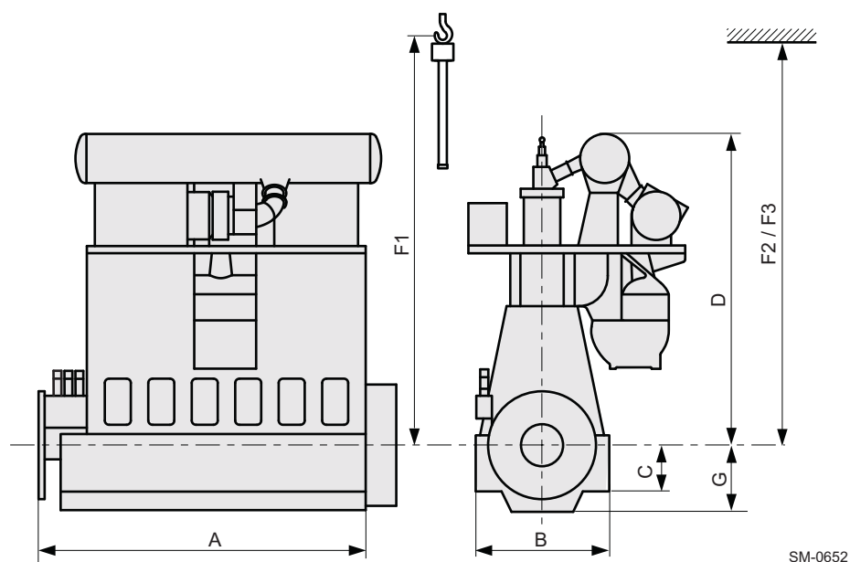
Figure 3-1 Engine dimensions
