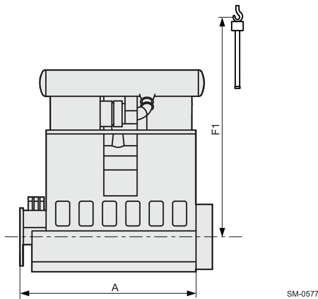
Figure 1-2 Principal engine dimensions
