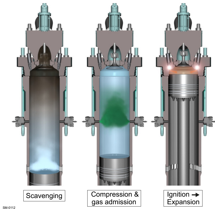
Figure 4-16 Lean burn with pilot ignition
