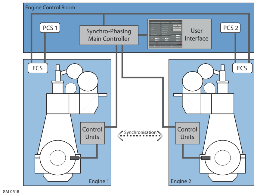
Figure 6-12 Synchro-Phasing system
