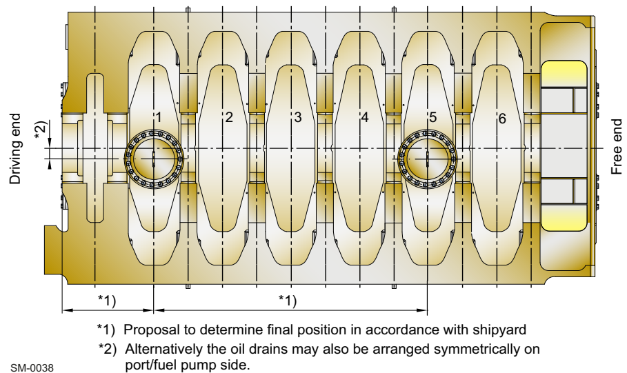
Figure 4-15 Arrangement of vertical lubricating oil drains for 6-cylinder engines
