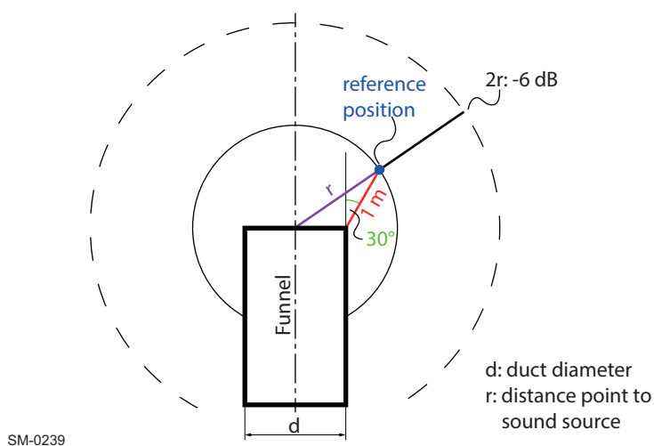
Figure 7-4 Exhaust noise reference point
