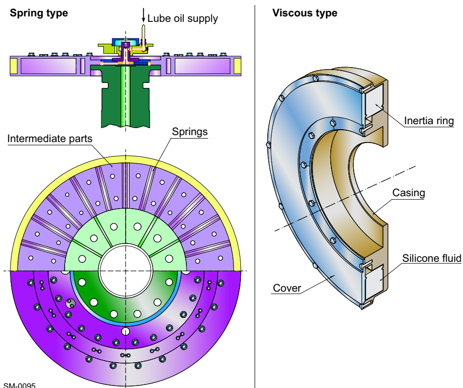
Figure 6-14 Vibration dampers (spring type and viscous type)
