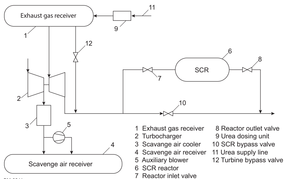
Figure 7-3 Low-pressure SCR with direct urea injection
