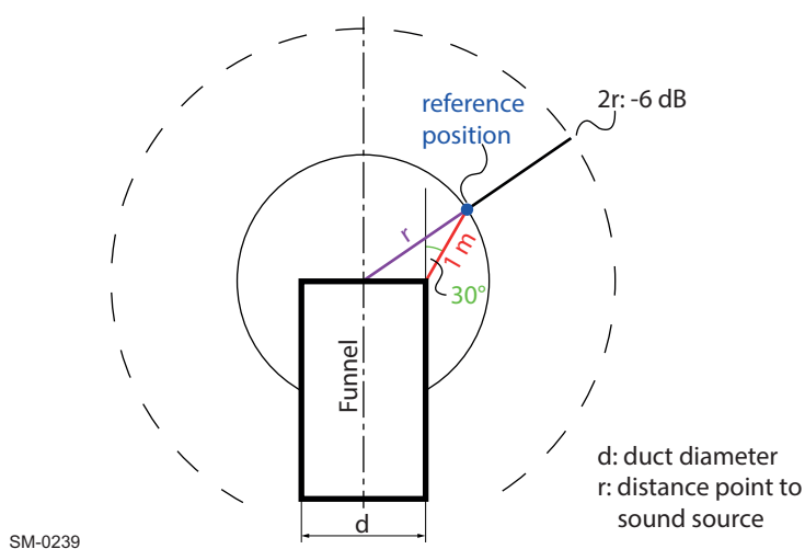
Figure 7-11 Exhaust noise reference point
