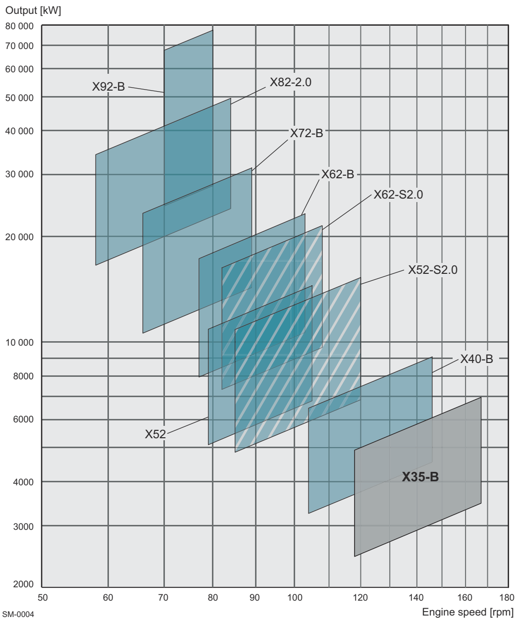
Figure 1-1 Power/speed range of WinGD diesel engines
