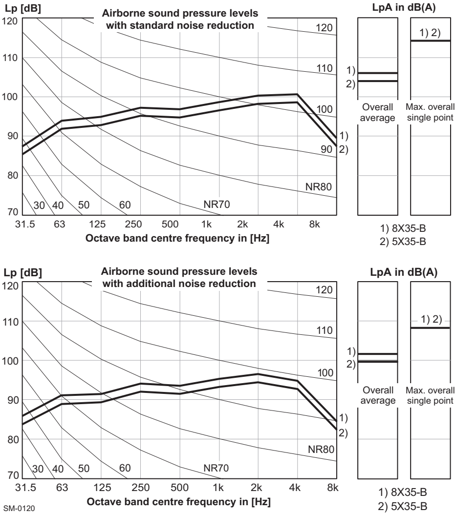
Figure 7-10 Sound pressure level at 1 m distance from engine
