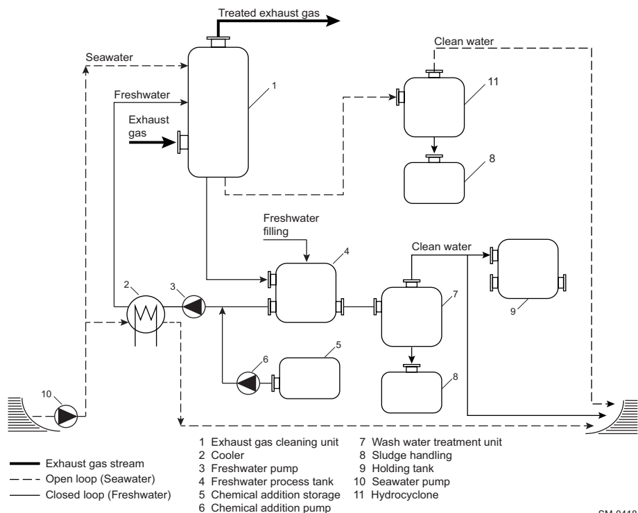
Figure 7-9 Hybrid scrubber system
