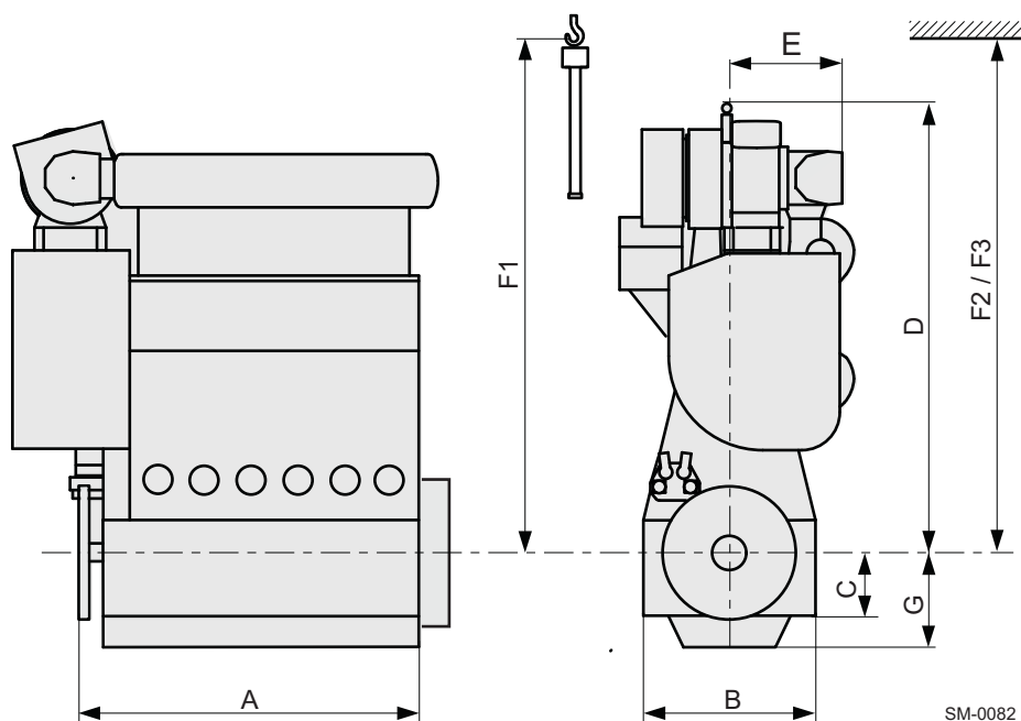
Figure 3-1 Engine dimensions
