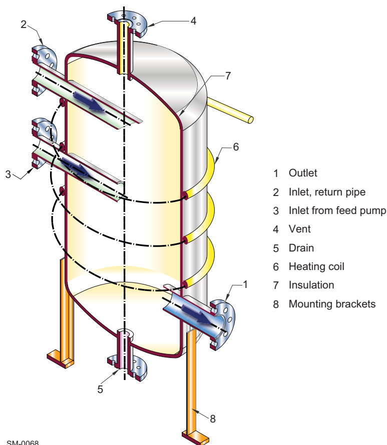
Figure 4-14 Mixing unit
