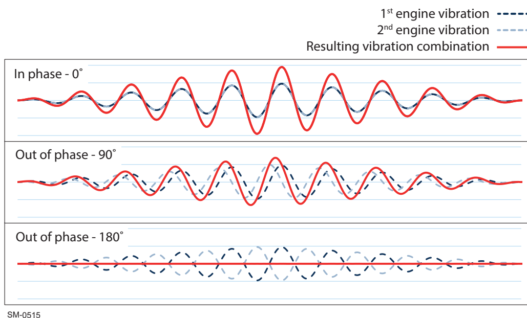
Figure 6-16 Resulting vibration from SPS combinations
