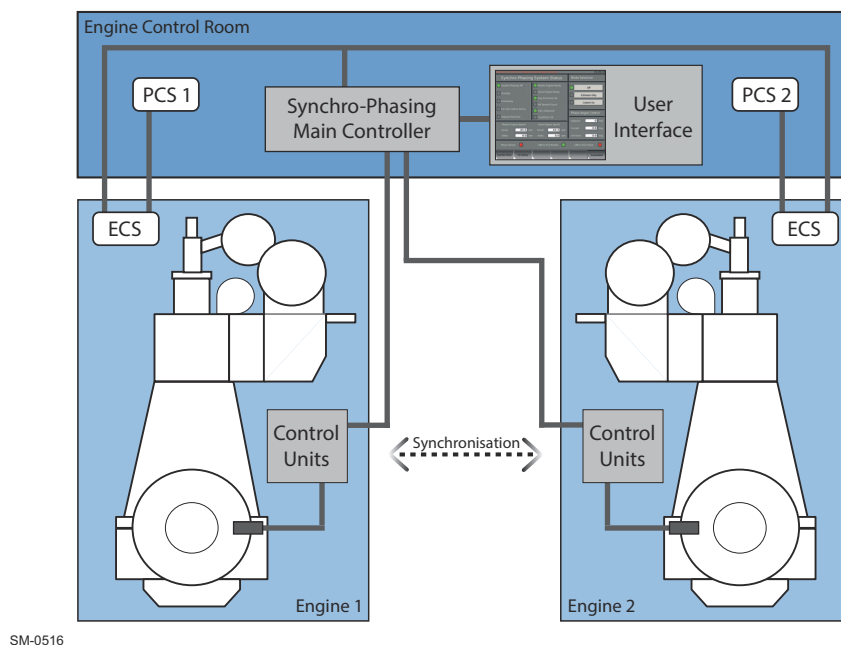
Figure 6-17 Synchro-Phasing system
