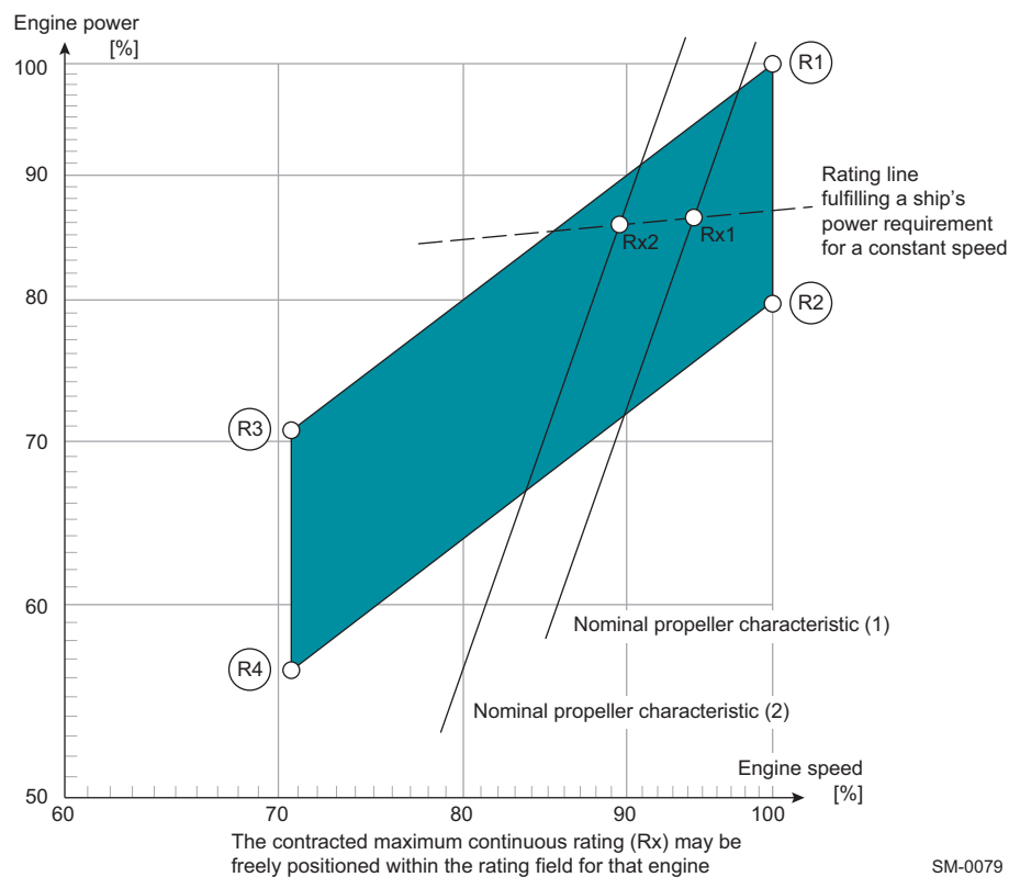
Figure 2-1 Rating field for the X35-B
