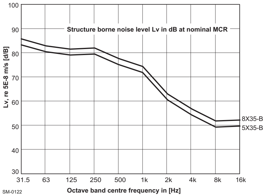
Figure 7-13 Structure-borne noise level at engine feet vertical
