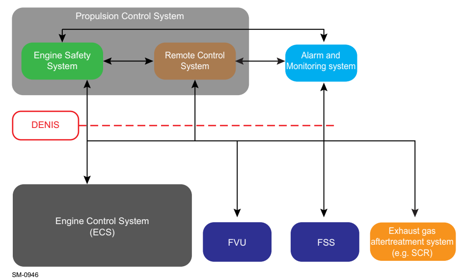
Figure 5-1 Engine automation architecture
