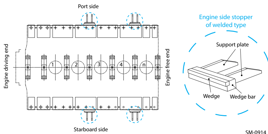
Figure 3-8 Welded type
