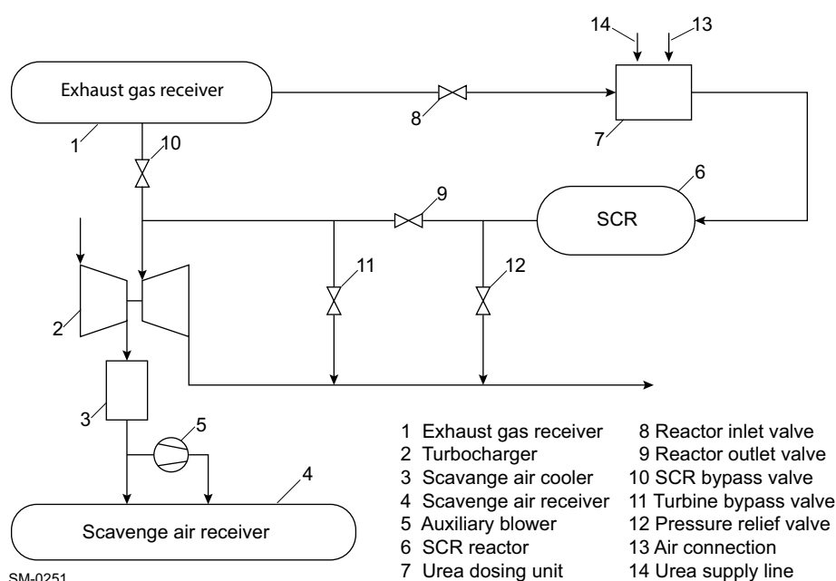
Figure 7-5 High-Pressure SCR
