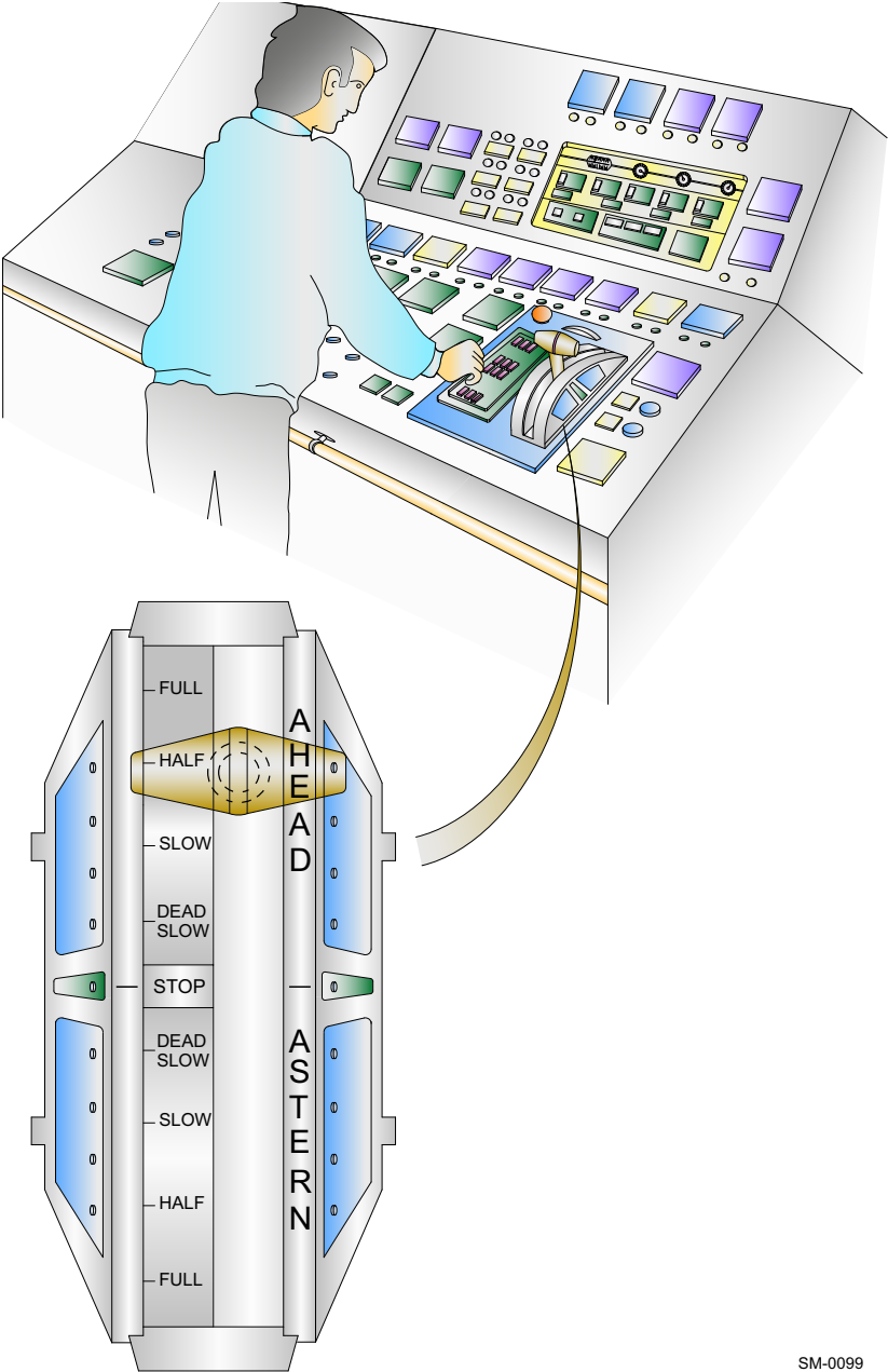
Figure 5-4 Propulsion control
