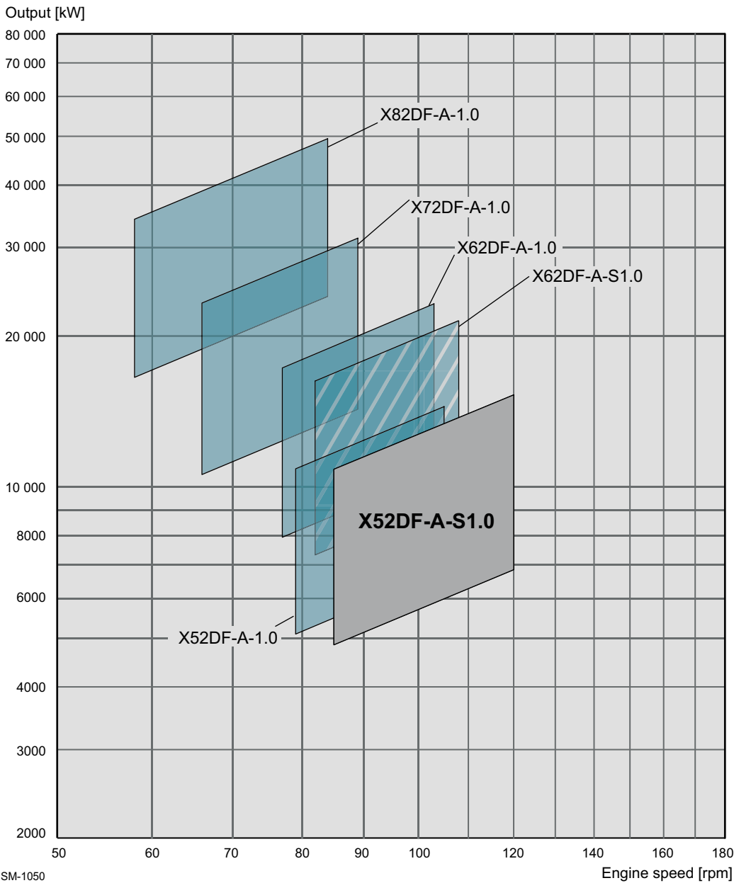
Figure 1-1 Power/speed range
