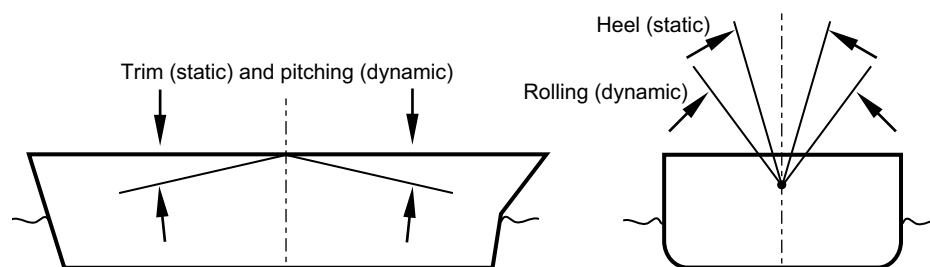
Figure 4-14 Inclination angles
