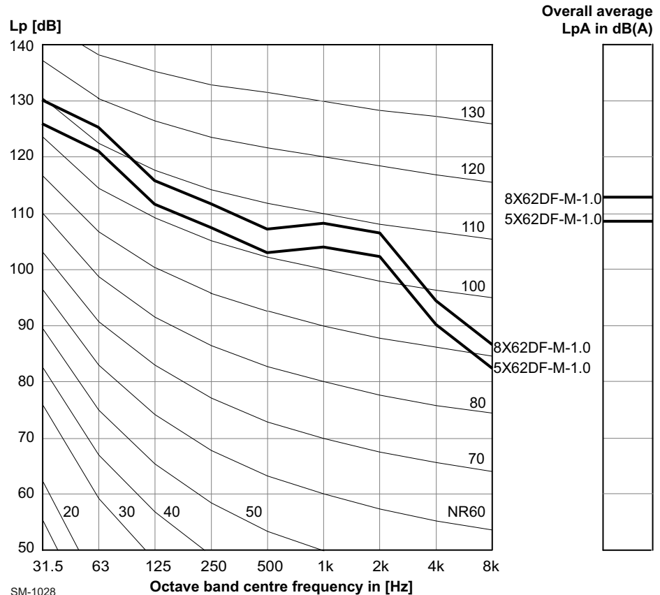
Figure 7-13 Sound pressure level at funnel top
