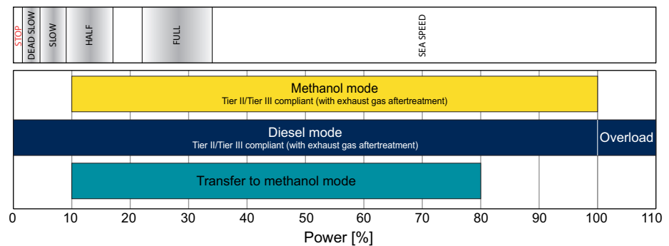
Figure 1-4 Operating modes of the X-DF-M engine
