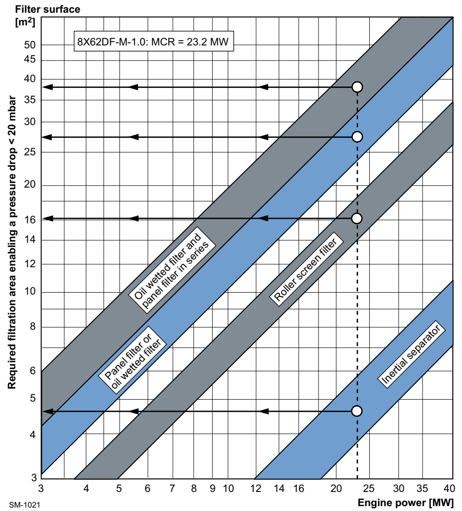
Figure 4-29 Air filter size (example for 8-cylinder engine)
