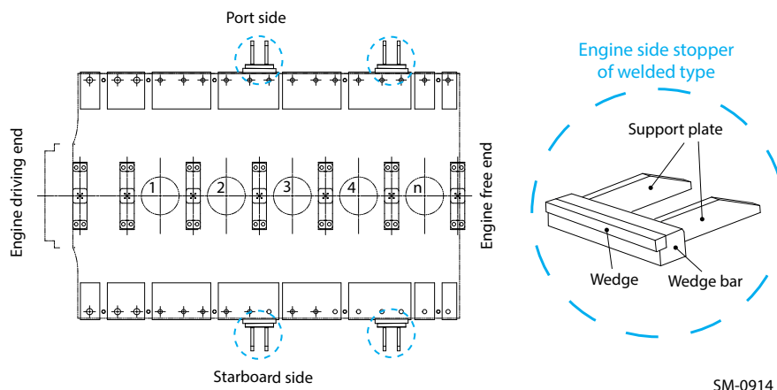
Figure 3-7 Welded type
