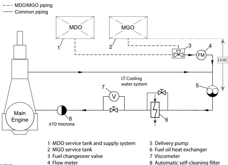
Figure 4-26 Fuel oil system: Arrangement with only MDO/MGO or MGO
