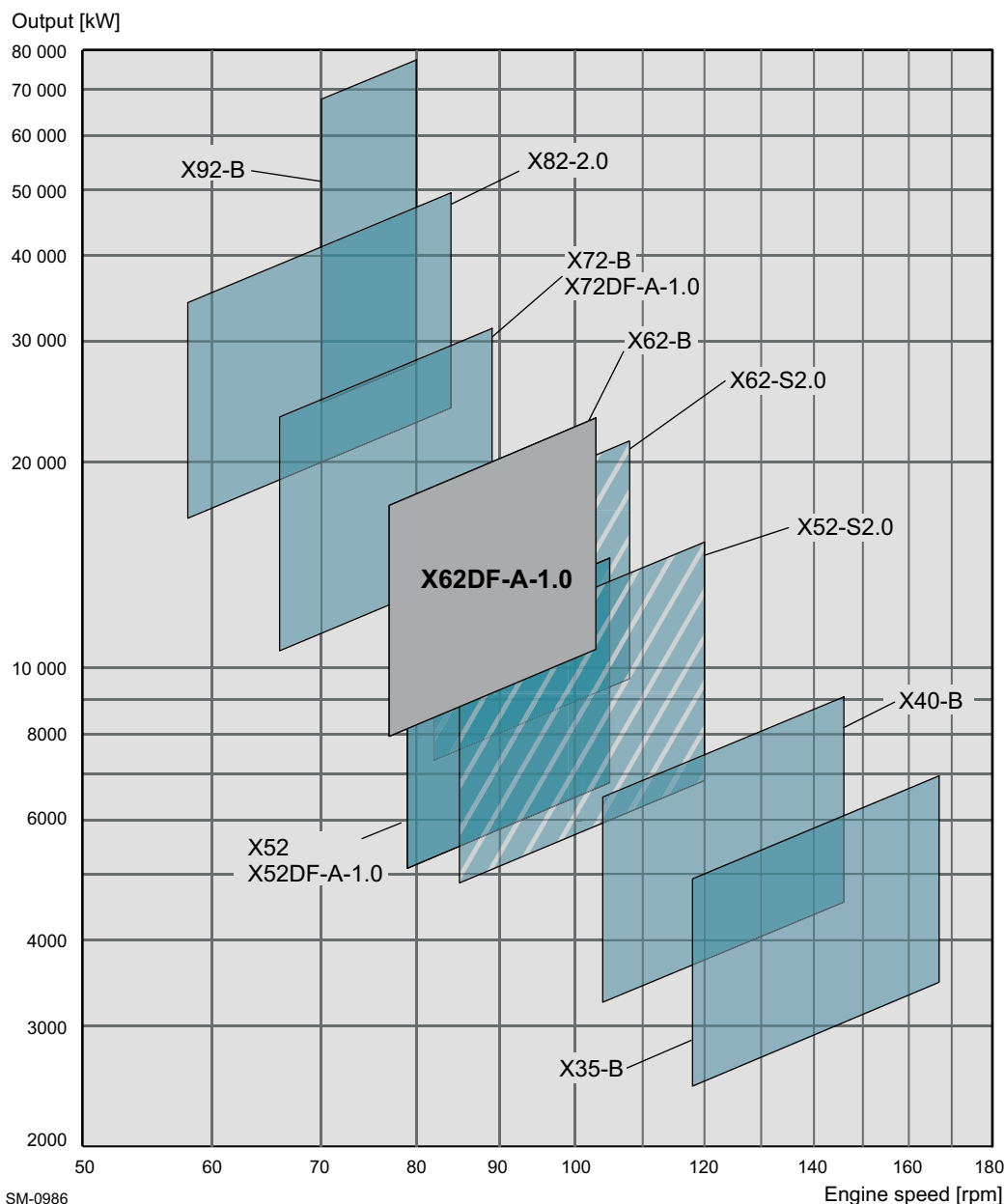
Figure 1-1 Power/speed range
