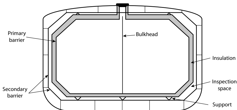
Figure 4-16 Section view of a free-standing Type A tank
