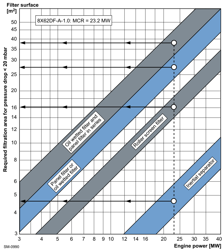
Figure 4-36 Air filter size (example for 8-cylinder engine)
