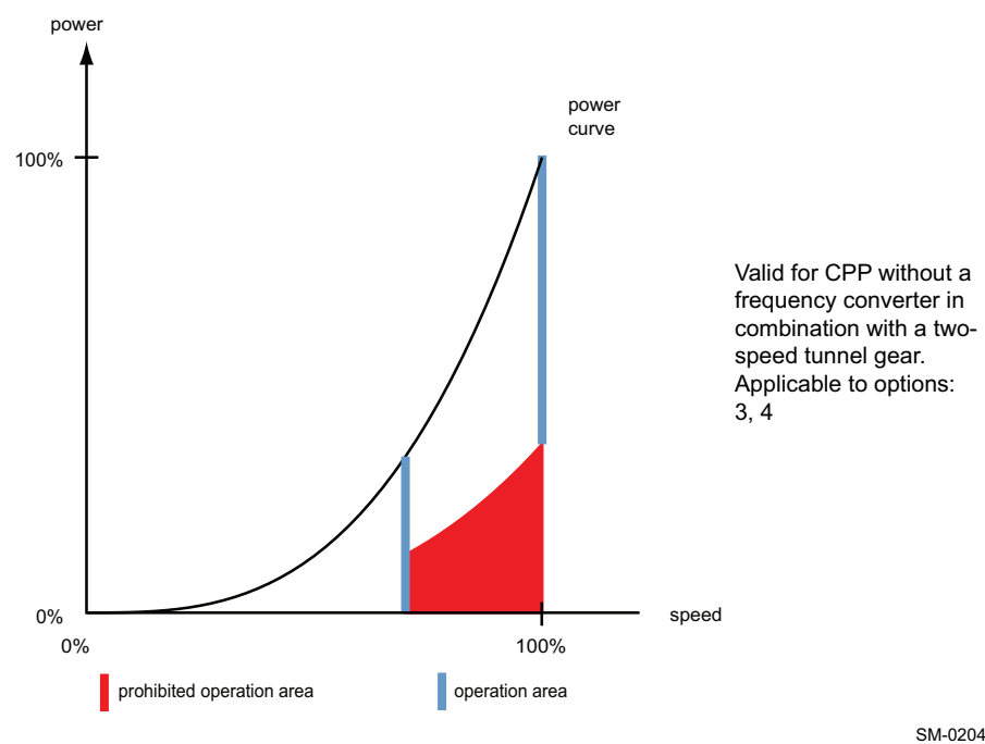
Figure 4-41 CPP with two fixed operation speeds without frequency converter
