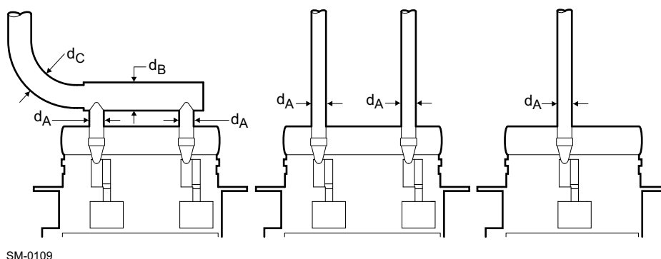
Figure 4-33 Determination of exhaust pipe diameter
