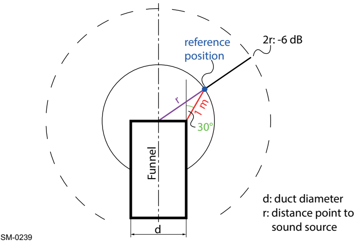
Figure 7-7 Exhaust noise reference point
